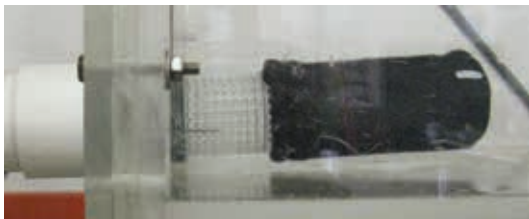
The two piece pre-filter fits snugly on a two inch outflow. The perforated tube goes onto the outflow pipe and a geotextile bag with draw strings fits over the tube.
